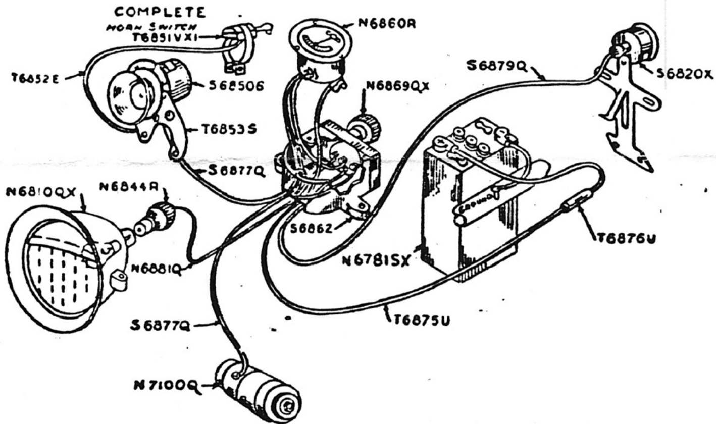
Wiring Diagram 1926
