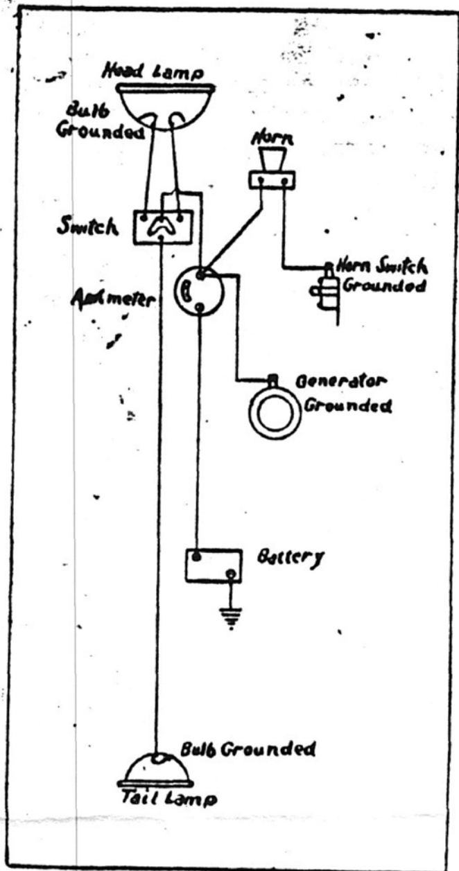
Wiring Diagram Indian Scout and Chief
