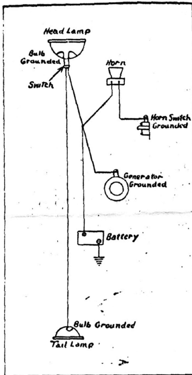
Wiring Diagram Indian Prince
